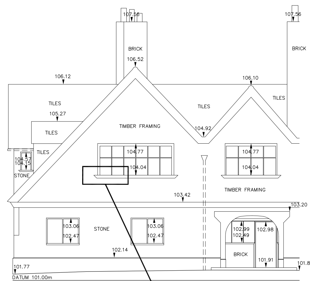
1:100 Standard Detail
