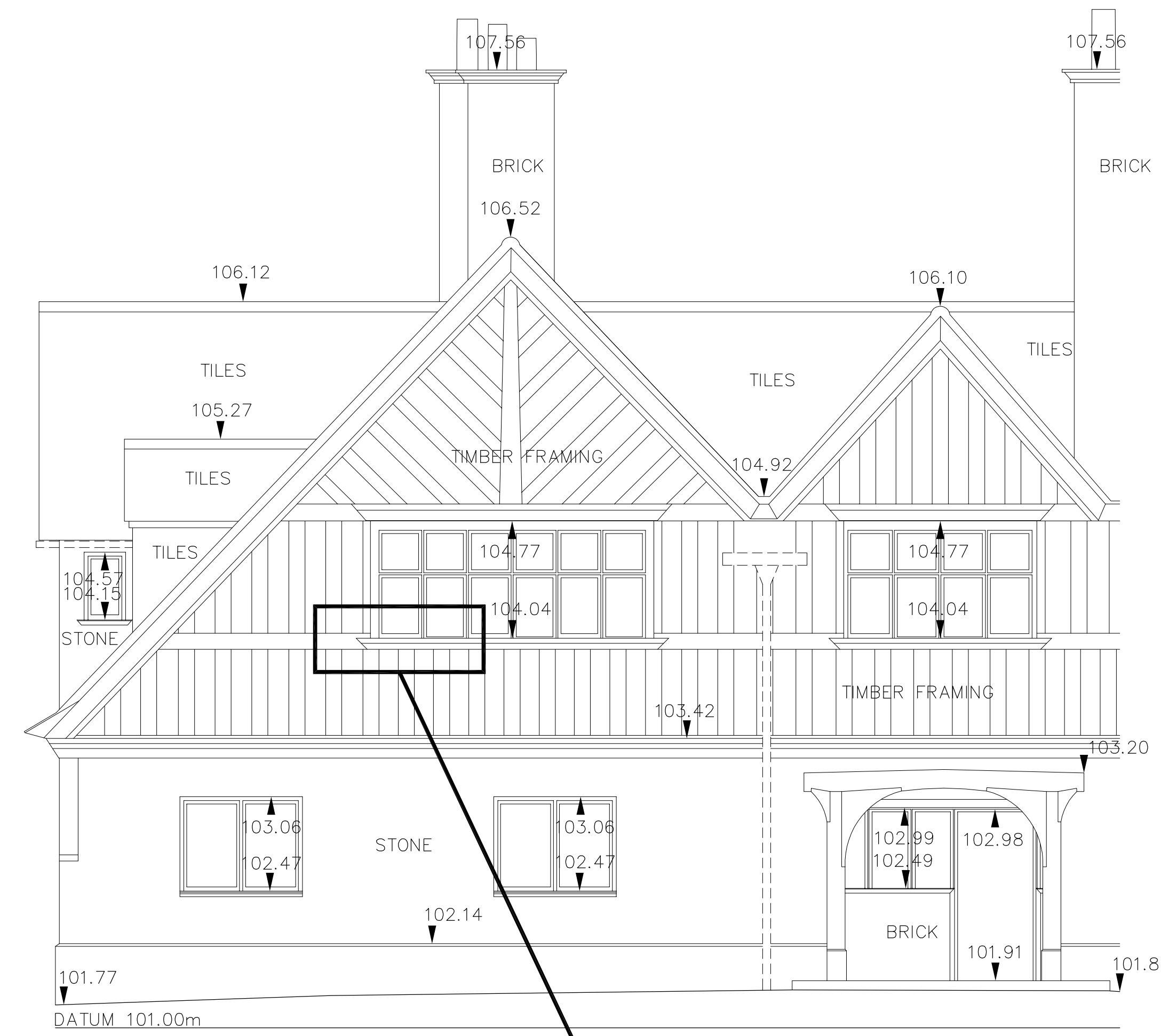
1:50 Standard Detail
