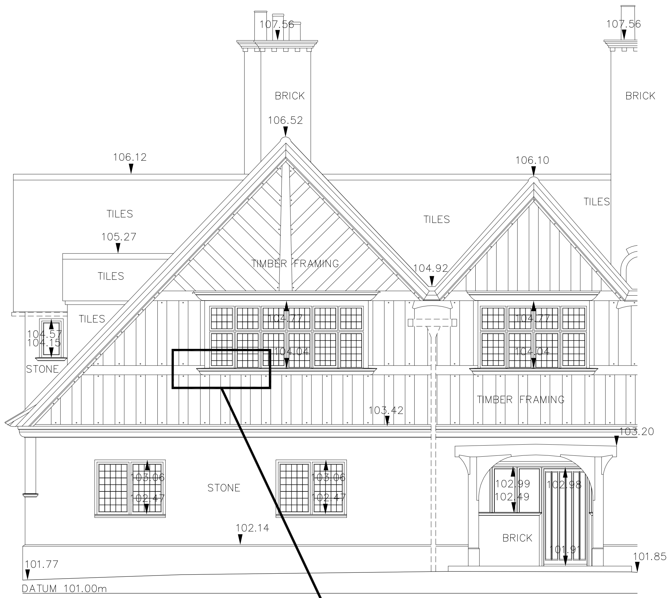
1:50 High Detail
