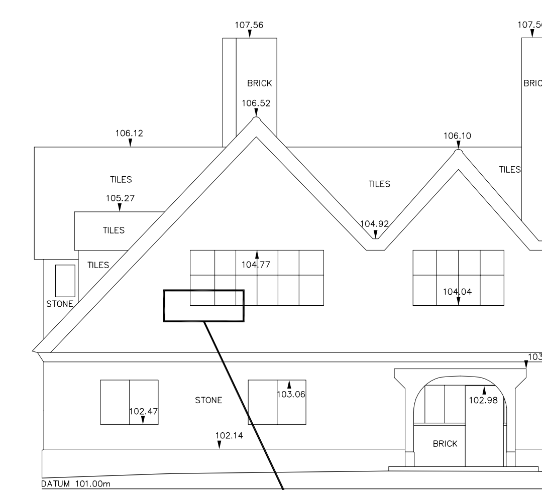
1:100 Basic Detail
