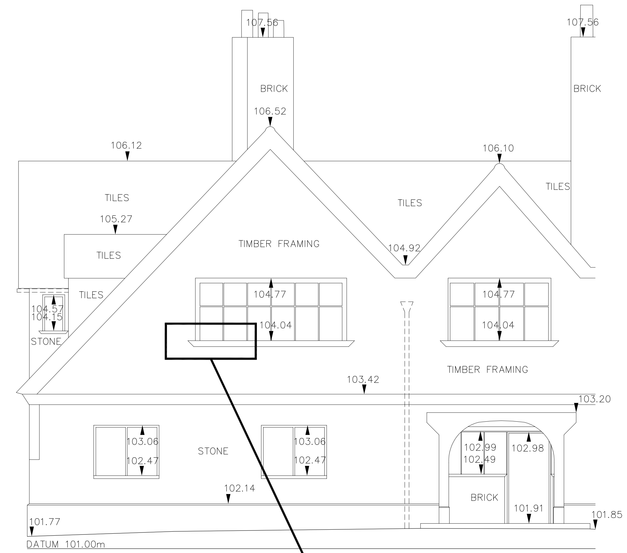
1:50 Basic Detail
