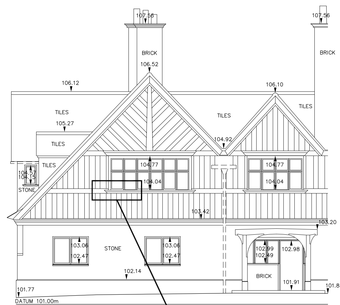
1:100 High Detail
